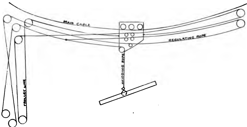
OVERHEAD LOG SKIDDER
