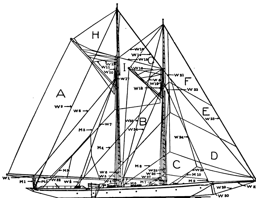
Sail and Rigging Plan of Yacht
