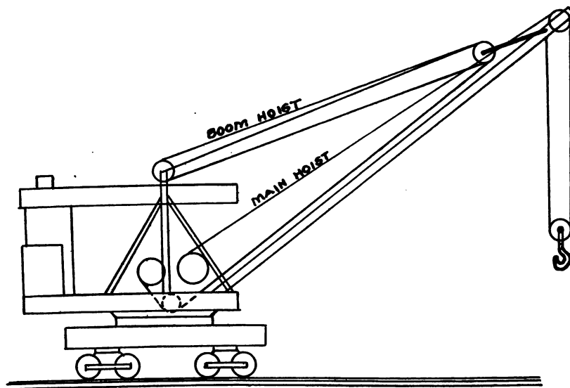
LOCOMOTIVE CRANE
